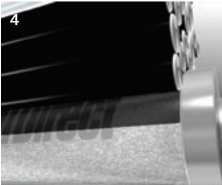
4 Then ink rollers are engaged and the plate is covered with ink.
