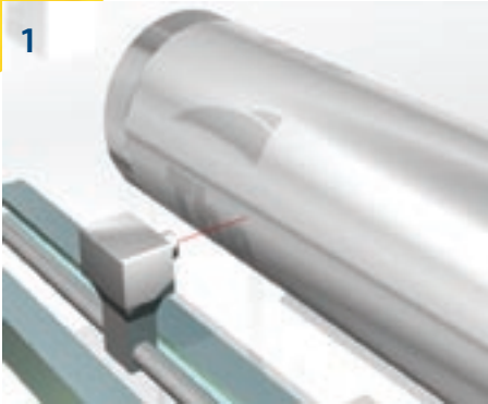
1 Laser energy writes the image to the ultra-thin coating. Coating in the image areas becomes non-soluble.
